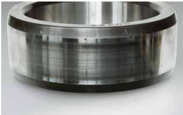
Photo 6.17.1 Part: Inner ring of a cylindrical roller bearing Symptom: Axial scratches on raceway surface Cause: Inclination of inner and outer rings during mounting
