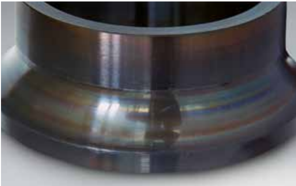
Photo 6.18.1 Part: Inner ring of an angular contact ball bearing Symptom: Bluish or purplish discoloration on raceway surface Cause: Heat generation due to poor lubrication
