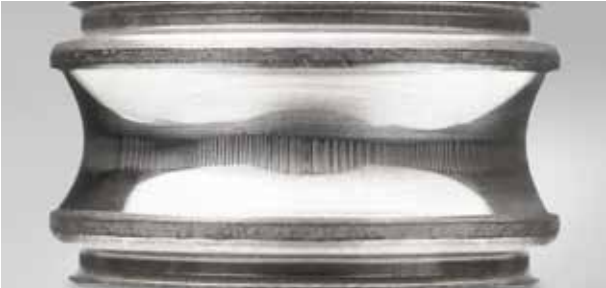
Photo 6.15.5 Part: Inner ring of a deep groove ball bearing Symptom: Fluting occurs on the raceway surface (high frequency)
