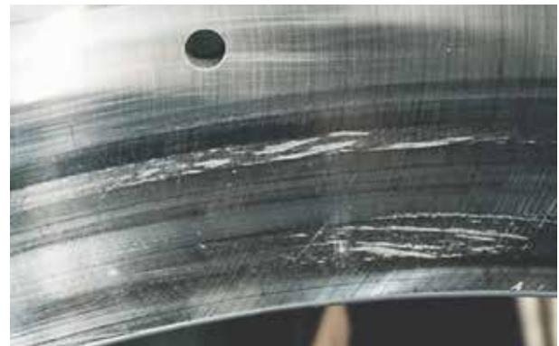
Photo 6.5.6 Part: Outer ring of Photo 6.5.5 Symptom: Partial smearing occurs circumferentially on raceway surface Cause: Poor lubrication
